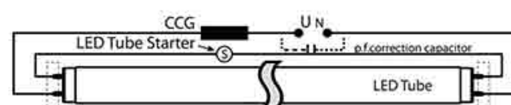
Wiring Diagram
